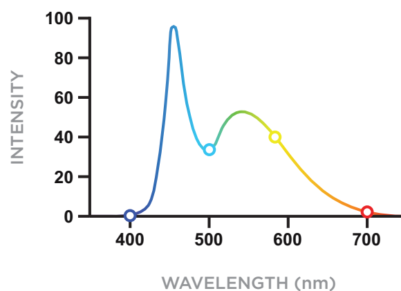
FIG.3 | Artificial cool white LED source spectrum
