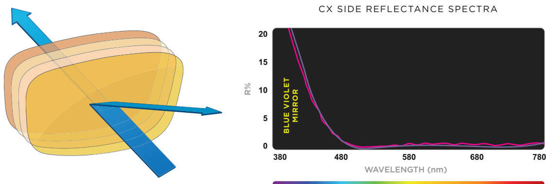
FIG. 6 | left: Blue mirror effect of an anti-reflective coating (AR) and its reflectance spectra (right)
